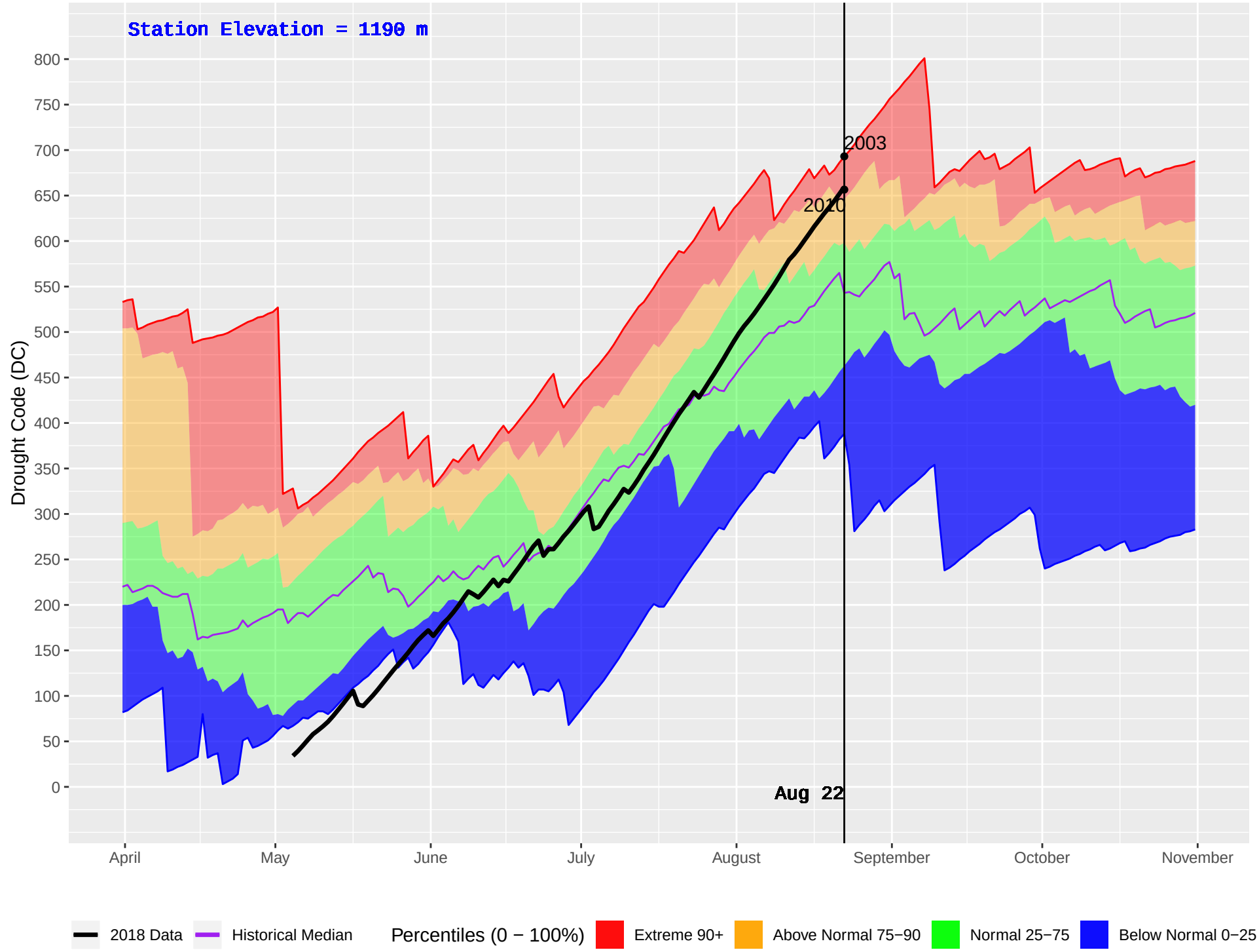
EMILY CREEK (425) : Historical (2002–2016) and Current (2018) Daily Drought Code (DC)
